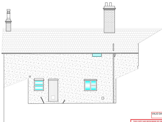
AS EXISTING NORTH ELEVATION (Scale 1:50)
